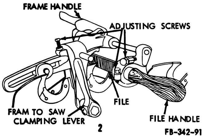
1 Tooth shaper. 2 File in frame for sharpening teeth.
